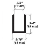
SC-658 U Channel
