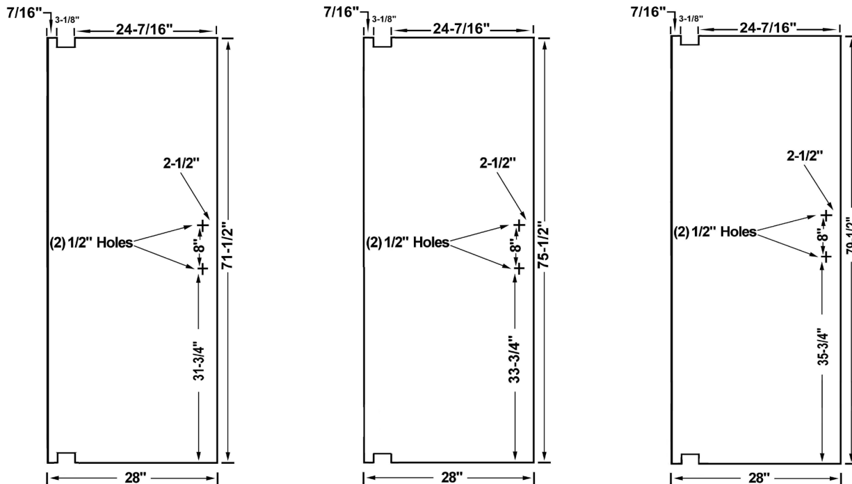
US Horizon Montreal Hinge Beveled pivot hinge, ceiling or curb mount.
